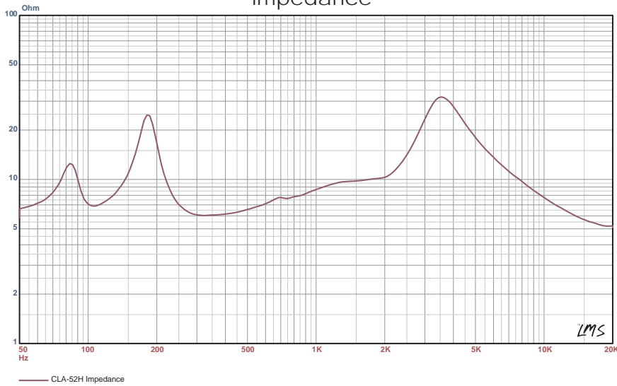
Impedance
