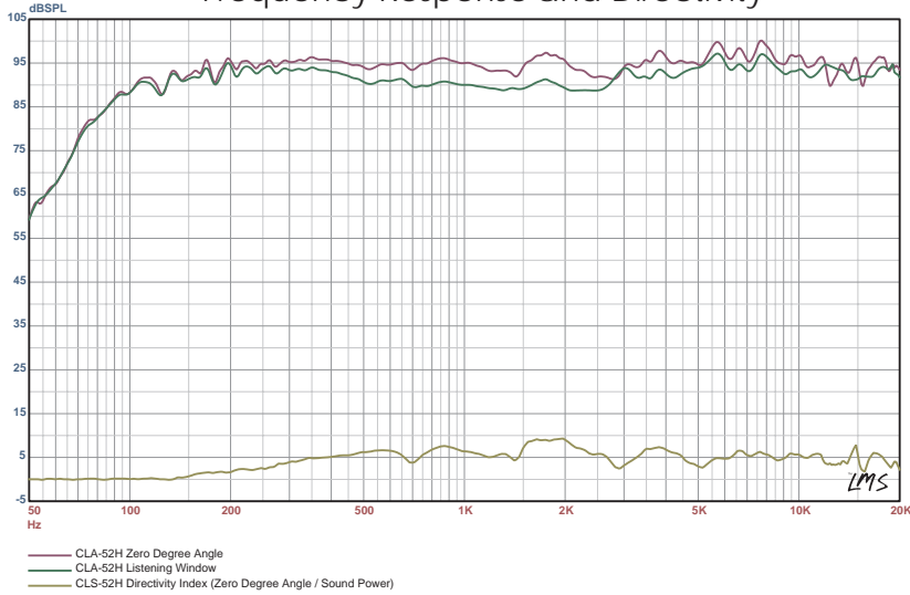
Frequency Response and Directivity
