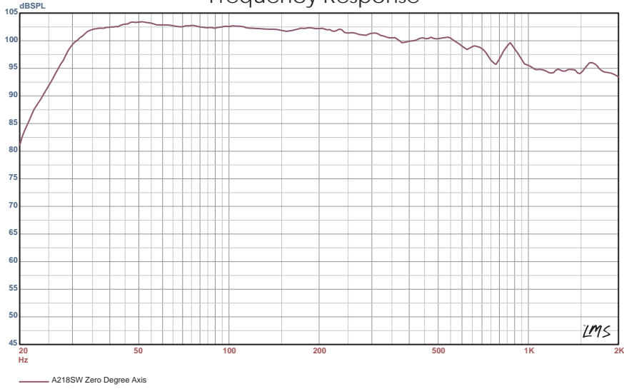
Frequency Response
