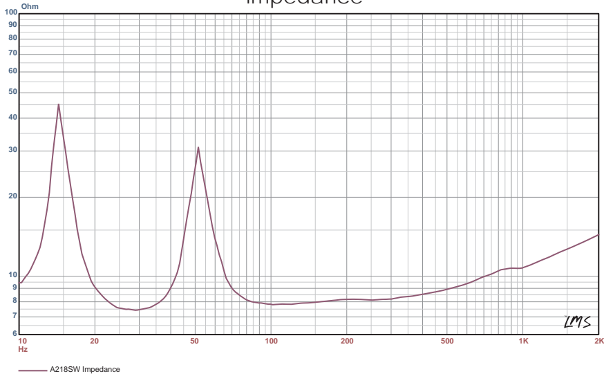
Impedance
